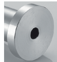
Smooth : SM Seal Face Roughness: Ra 3.2 to 6.3 Micrometer
